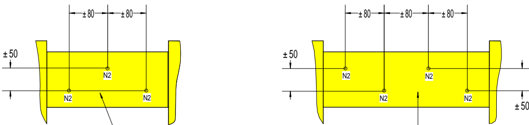
Bottom view
